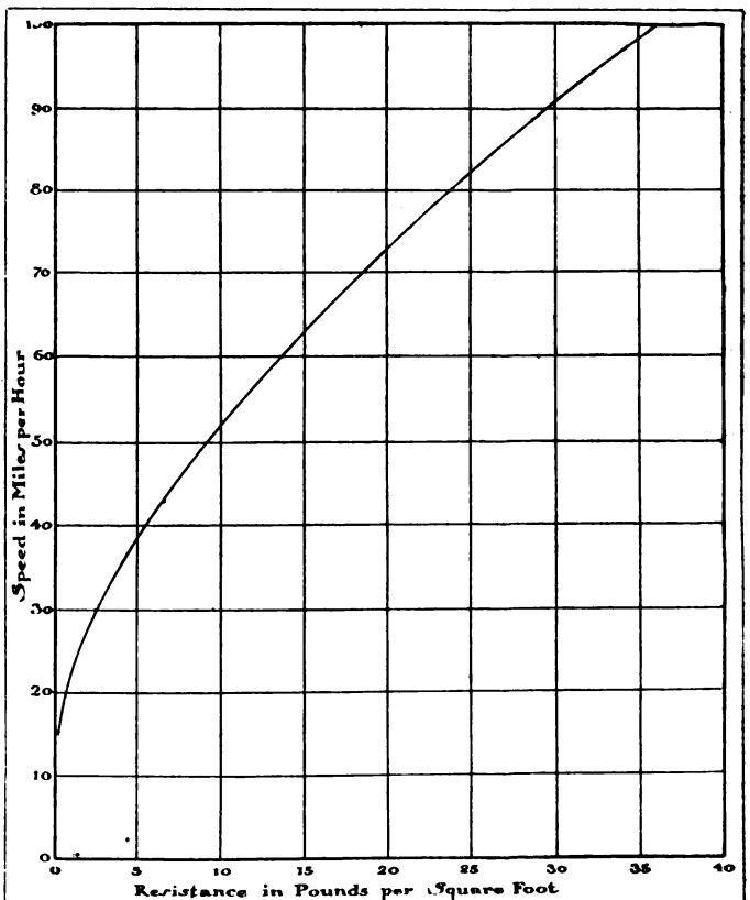
Fig. 10.—Curve showing resistance of bodies through air.
